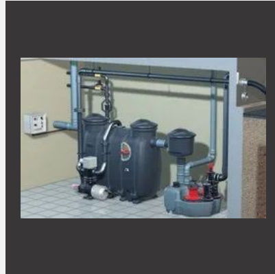
Grease separator Euro E+S PV
