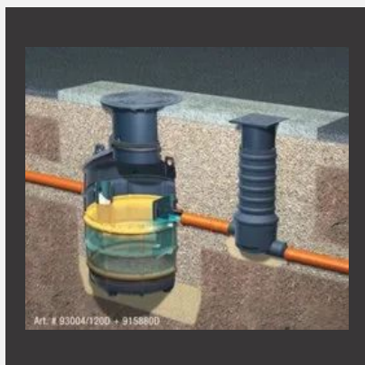
Grease separator Euro G according EN 1825-1 NS 1/2/4 for underground installation
