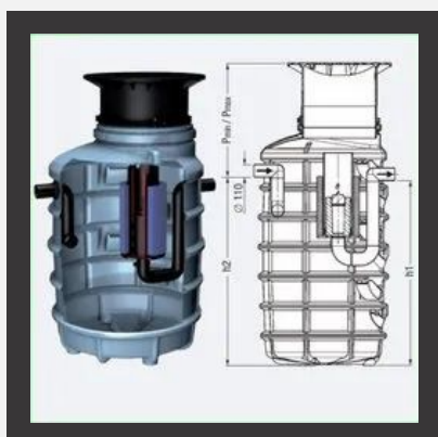
Coalescence separator NS 3/6 according to EN 858, Class I
