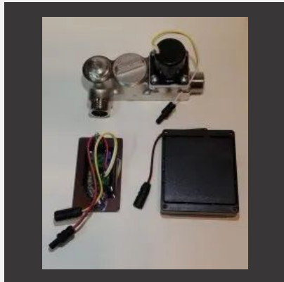
Roca Urinal Sensors
